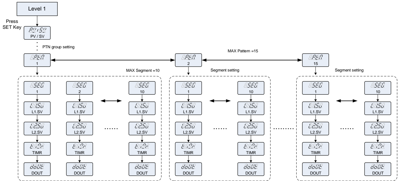
Program edit flow-chart
